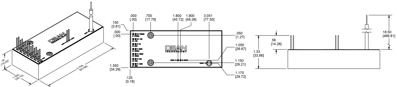
Dimensions in inches [mm]
